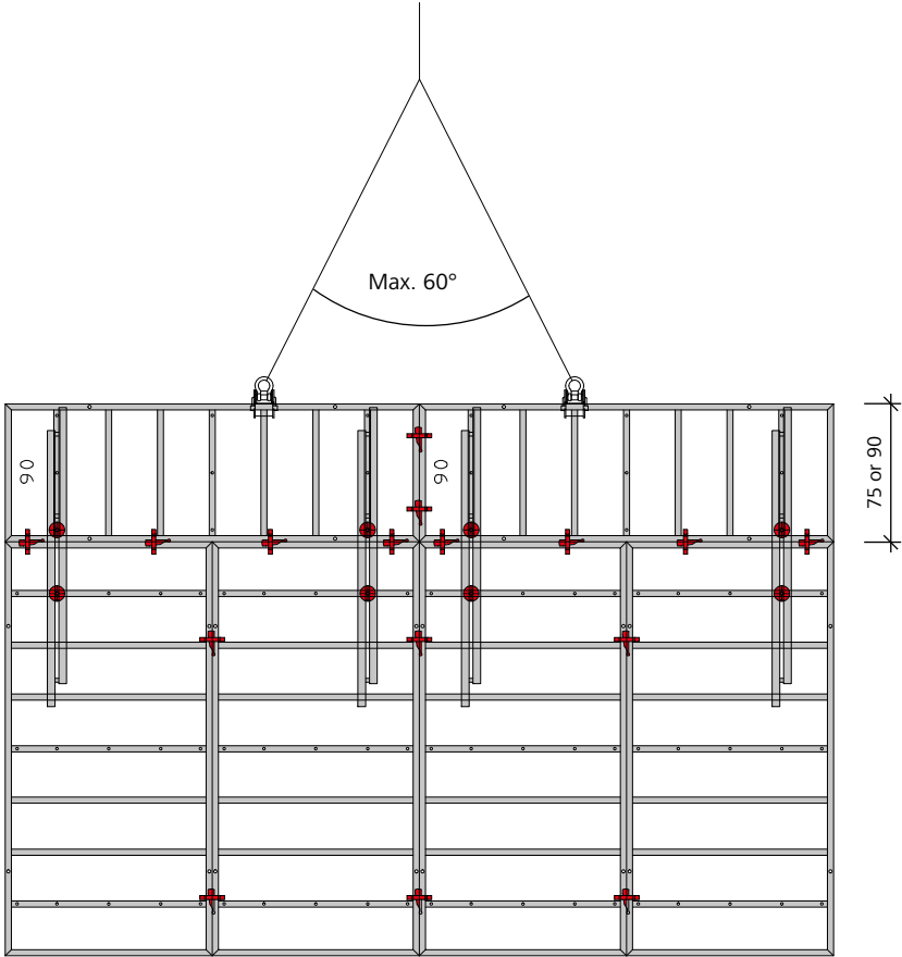
Fig. 58.3 Height extension with horizontal StarTec panels 270/90 or 270/75
