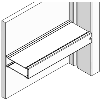
Fig. 54.3 Aluminium cross stiffener (with grip profile)
