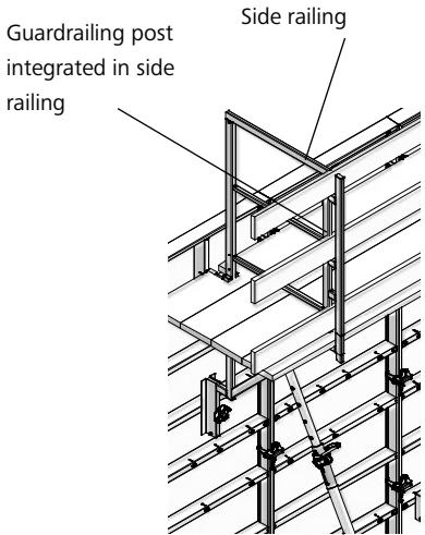
Fig. 21.5 Side railing
