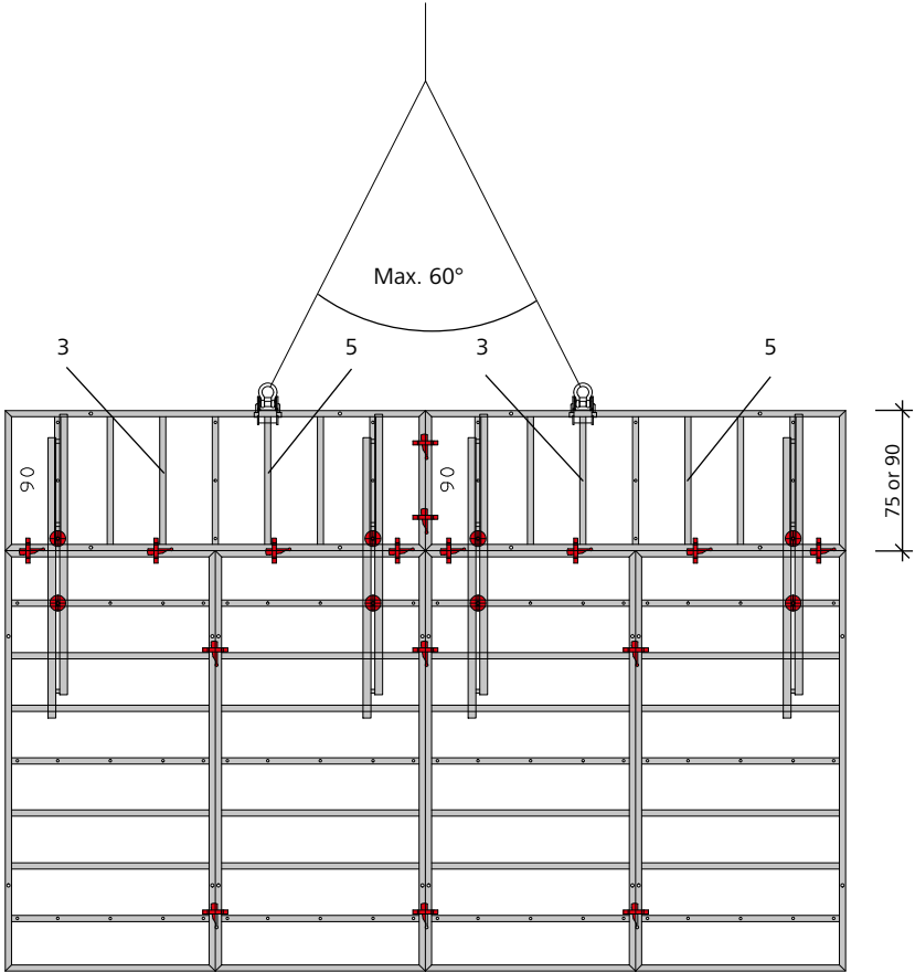
Fig. 57.3 Height extension with horizontal StarTec panels 270/90 or 270/75
