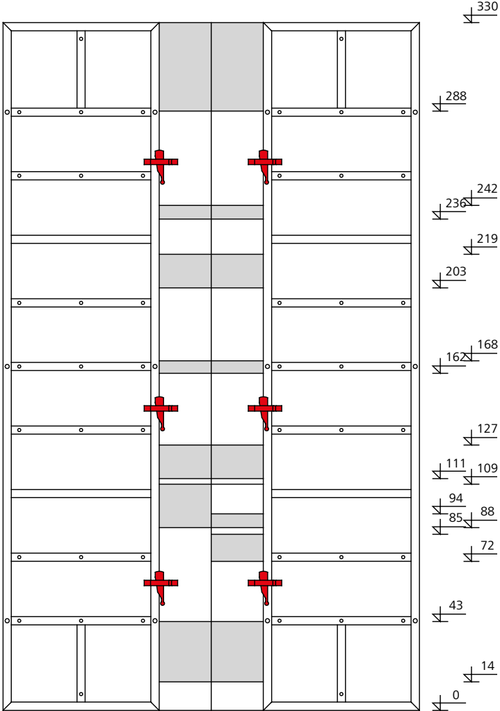
Fig. 34.1 ST stripping corner 330/25
