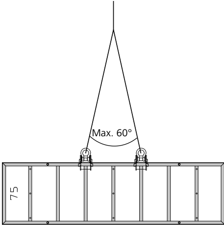
Fig. 58.2 StarTec panel 270/75
