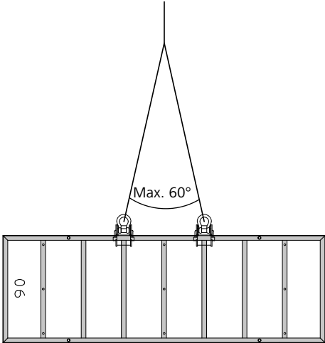
Fig. 58.1 StarTec panel 270/90
