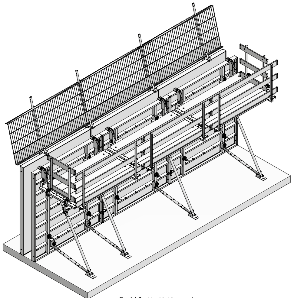
Fig. 4.1 Double-sided formwork
