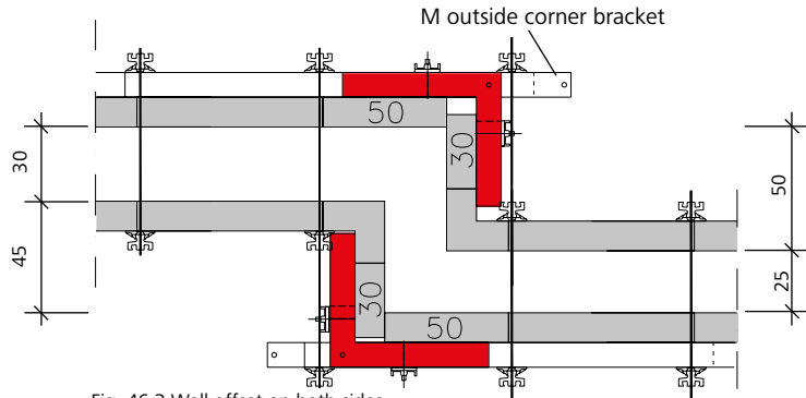
Fig. 46.3 Wall offset on both sides
