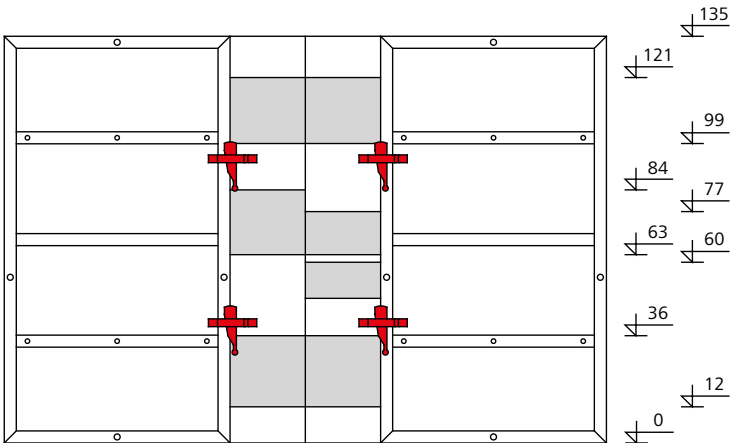
Fig. 35.2 ST stripping corner 135/25
