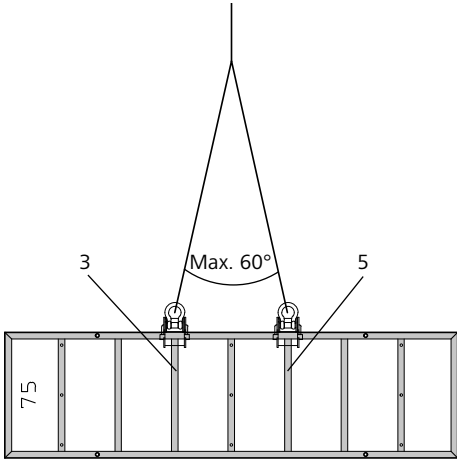
Fig. 57.2 StarTec panel 270/75
