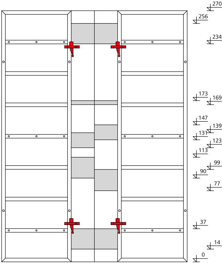
Fig. 35.1 ST stripping corner 270/25
