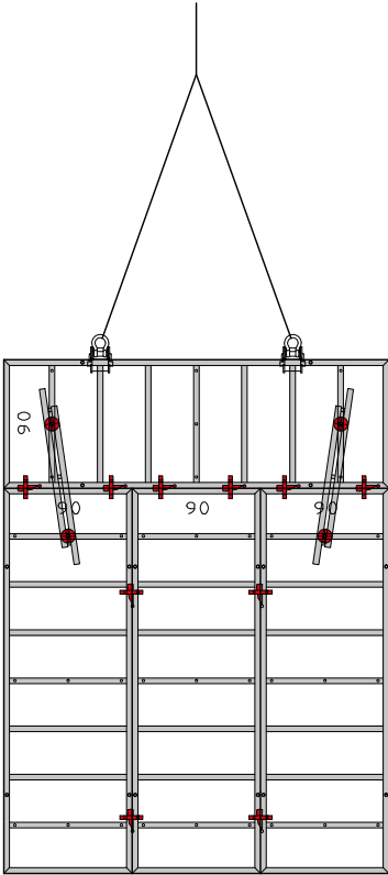
Fig. 59.2 AluStar or StarTec unit, height-extended with horizontal AluStar panel 270/90
