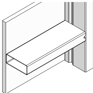
Fig. 54.4 Steel cross stiffener (without grip profile)
