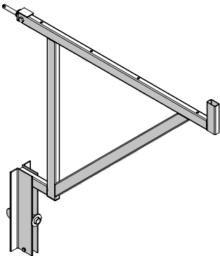
Fig. 21.2 Walkway bracket 90
