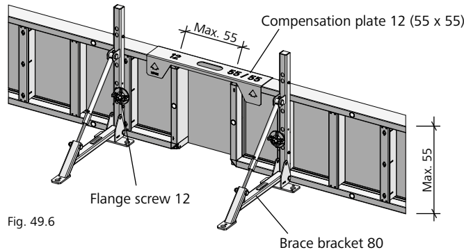
Brace bracket 80
