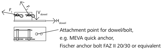
Fig. 18.2 Double-jointed foot plate
