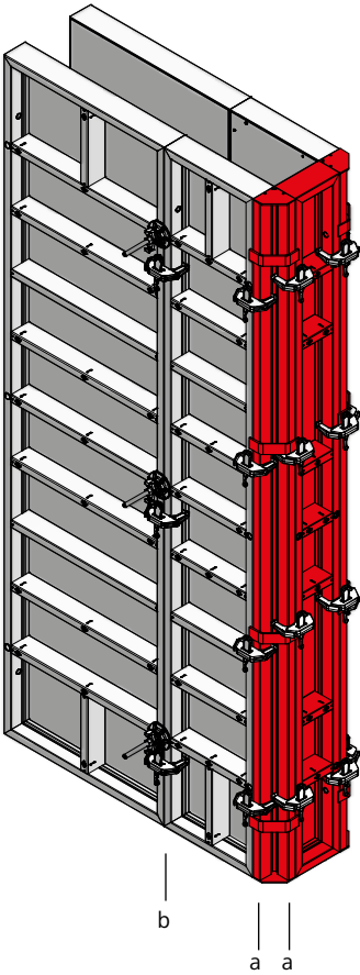
Fig. 44.1 Height 330 cm
