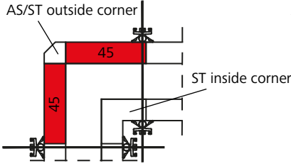
Fig. 30.1 Wall thickness 20 cm
