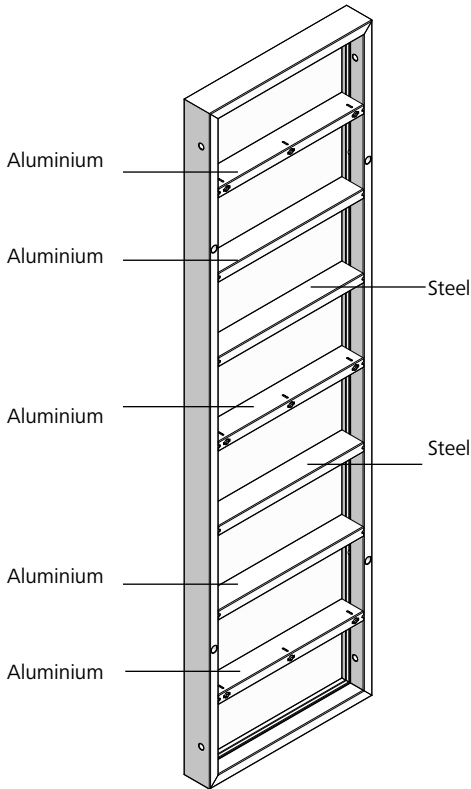
Fig. 54.1 StarTec panel 270/90 and 270/75 built until 2006
