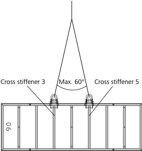
Fig. 57.1 StarTec panel 270/90
