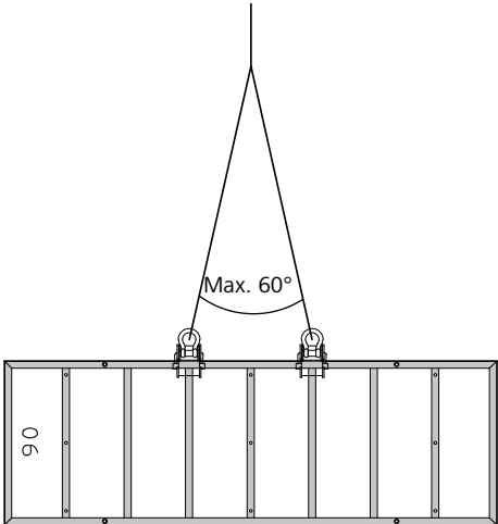
Fig. 59.1 AluStar panel 270/90
