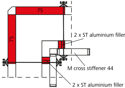
Fig. 30.4 Wall thickness 40 cm
