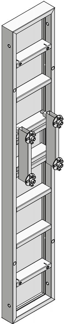
Fig. 68.6 Panel with concreting window
