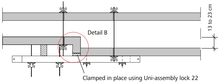
Fig. 46.2 Wall offset
