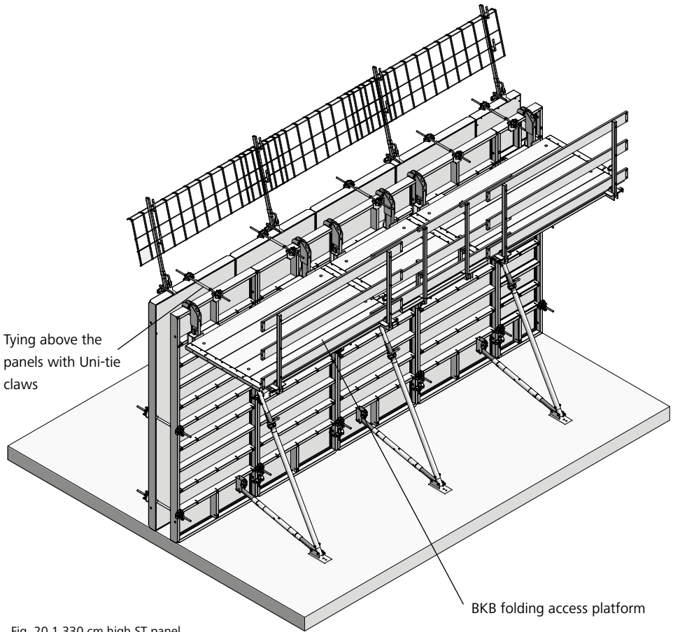
Fig. 20.1 330 cm high ST panel
